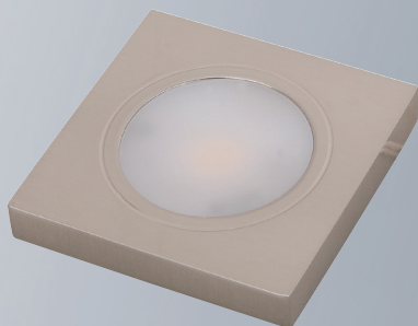
Item No.:202778-SI Lumen:250LM 12VDC,3.6W, 9xLEDs*SMD2835 Size:65*65*10mm Material: Alum, Plastic
